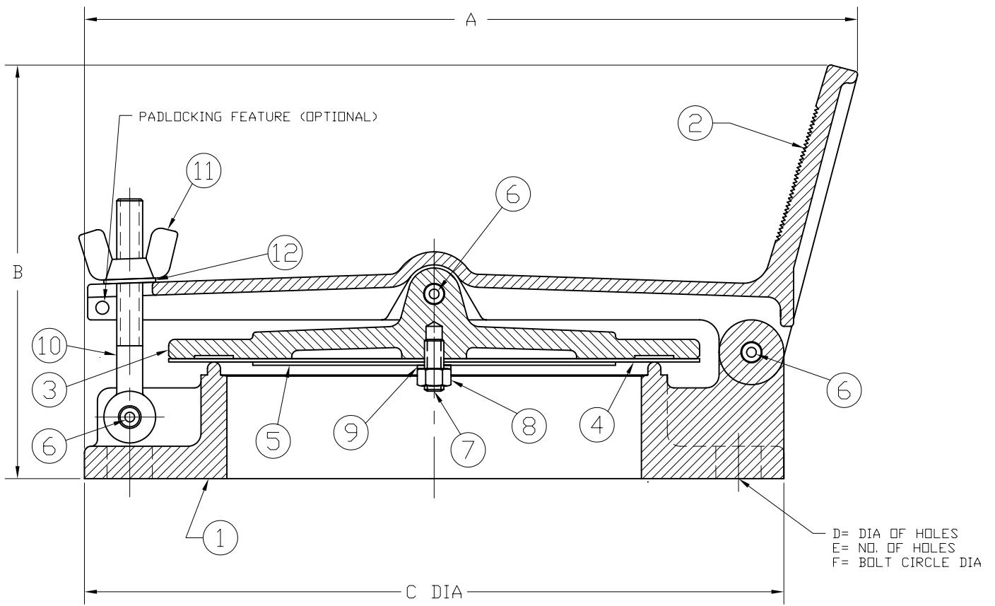
MODEL 6100 GAUGE HATCH
