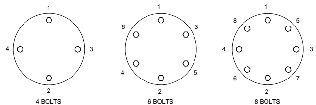
Figure 'B' EXAMPLE OF BOLT TORQUE SEQUENCE
