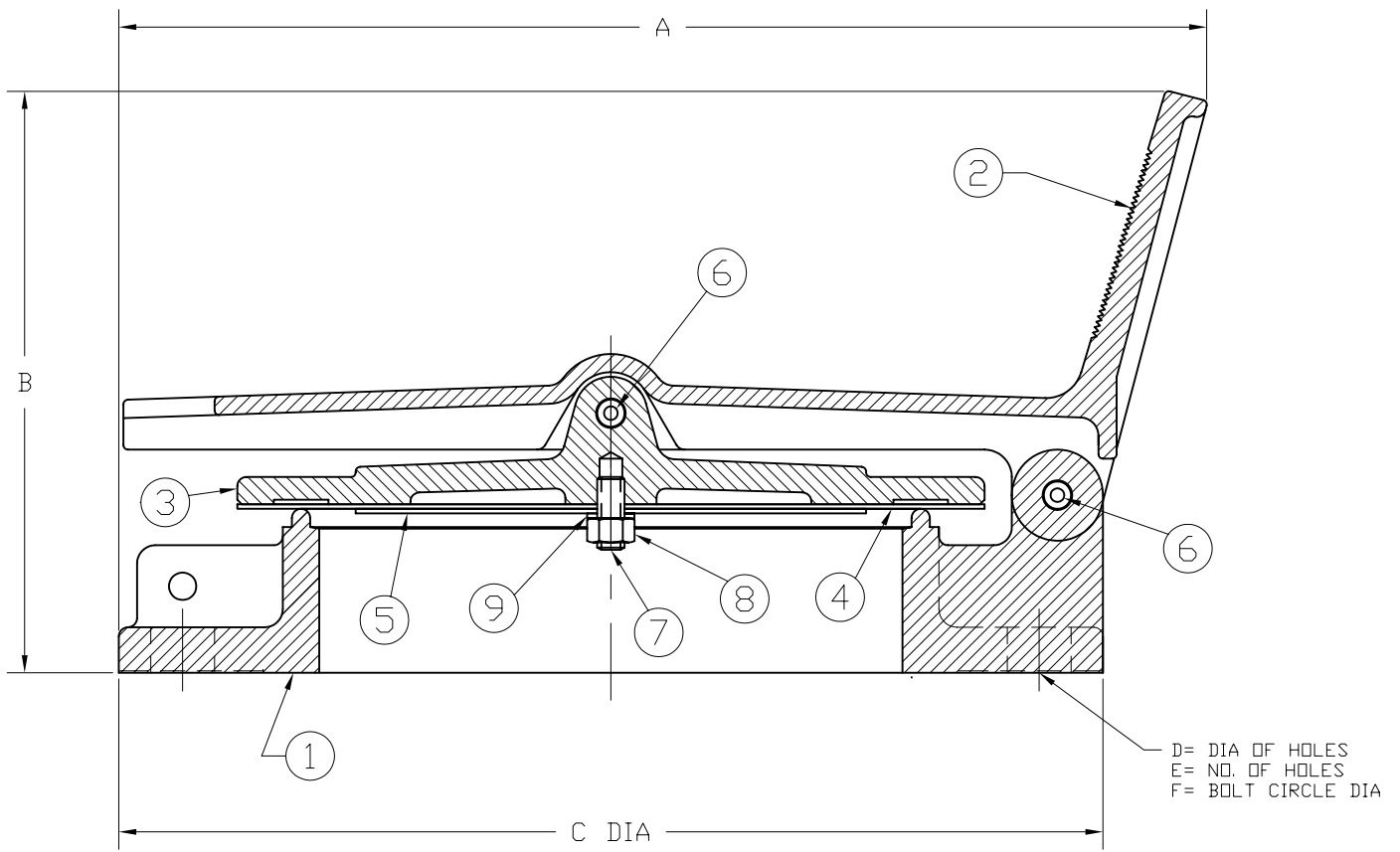
MODEL 6000 GAUGE HATCH
